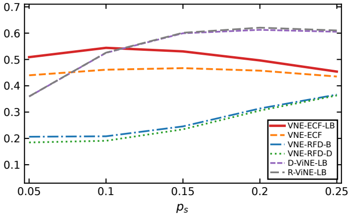
Average Link Utilization
